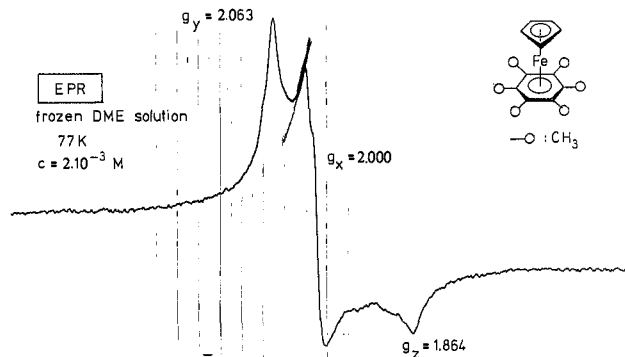
Figure 4. EPR spectrum of CpFeC 6 Me 6 .
