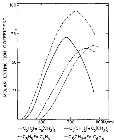
Figure 3. Optical spectra of d 7 CpFe(arene) in DME in the visible region.
