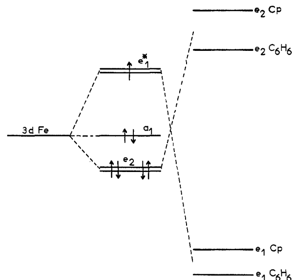
Figure 5. Molecular orbital diagram (d set) for d 7 CpFeC 6 H 6 . Note that ring levels are raised upon permethylation.
